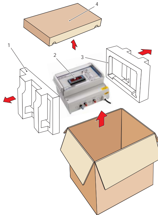
Figure 2 Unpacking Method
