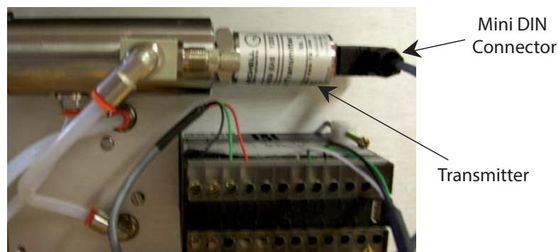
Figure 15 Sensor Removal
