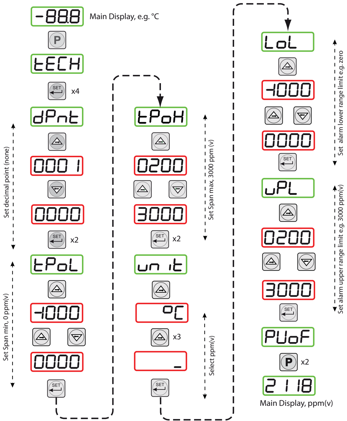
Figure 13 Set-up Monitor (to read ppm v )
